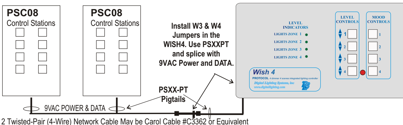
Figure 6 Typical System Powered By An External Transformer
