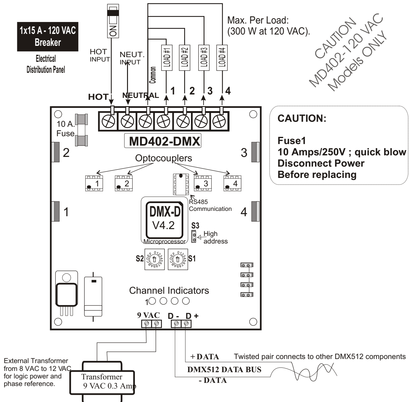
Figure 7 - MD402-DMX-120 Typical 120 VAC Wiring.
