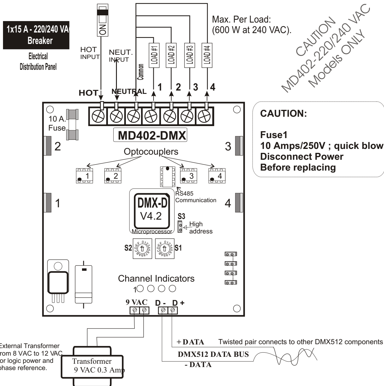
Figure 7 - MD402-DMX-240 Typical 220/240 VAC Wiring.
