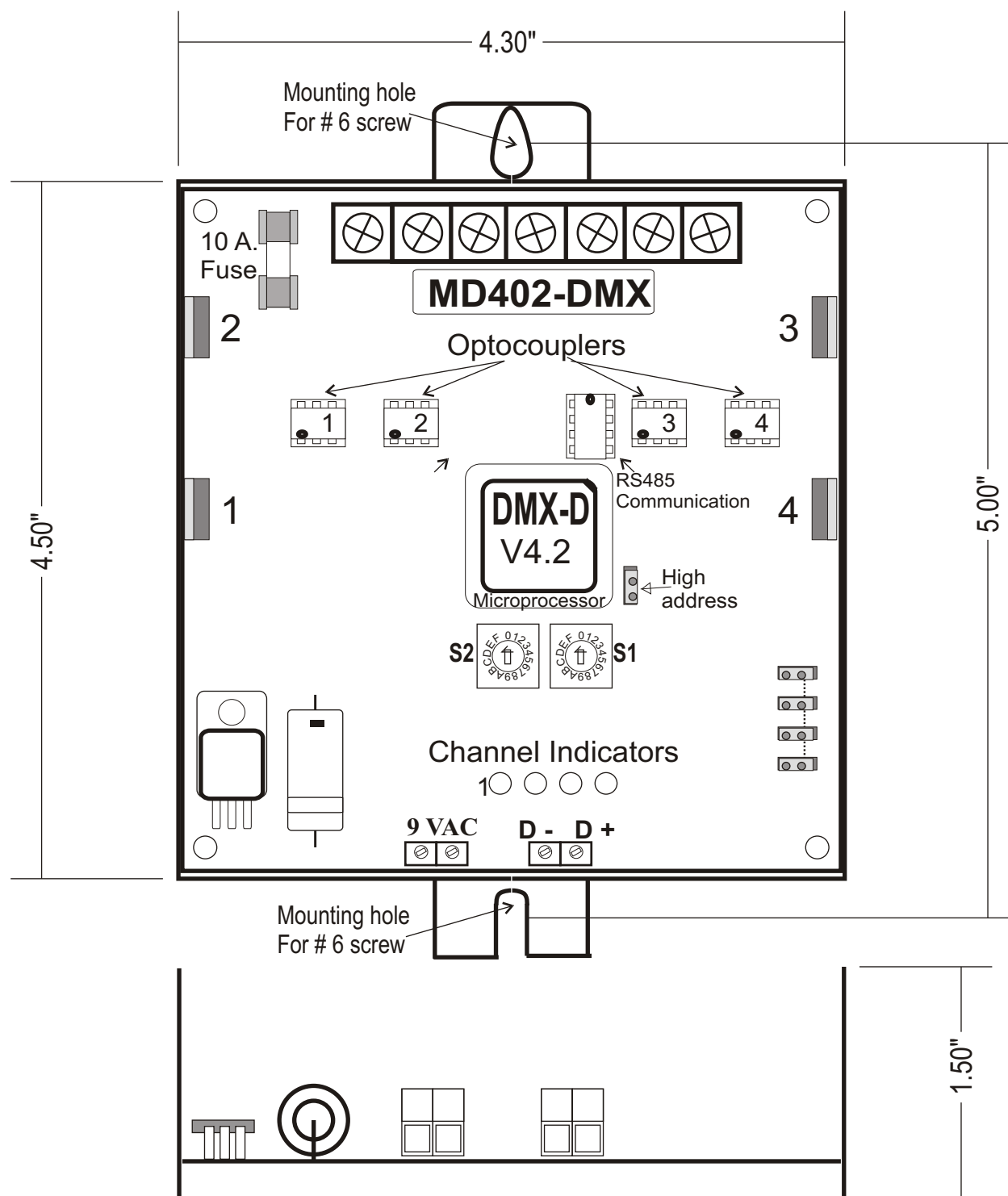
Figure 3 - MD402-DMX Dimensional Diagram
