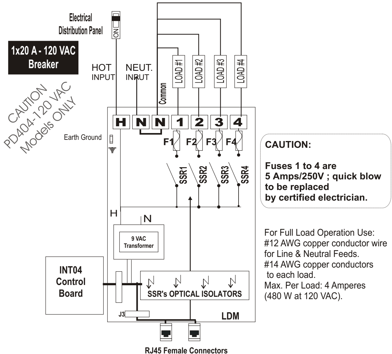
Figure 7 - PD404 Typical 120 VAC Wiring.
