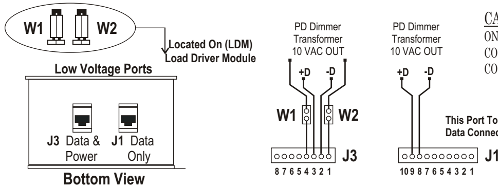
Figure 5 - Typical System Powered By a PD Dimmer Module
