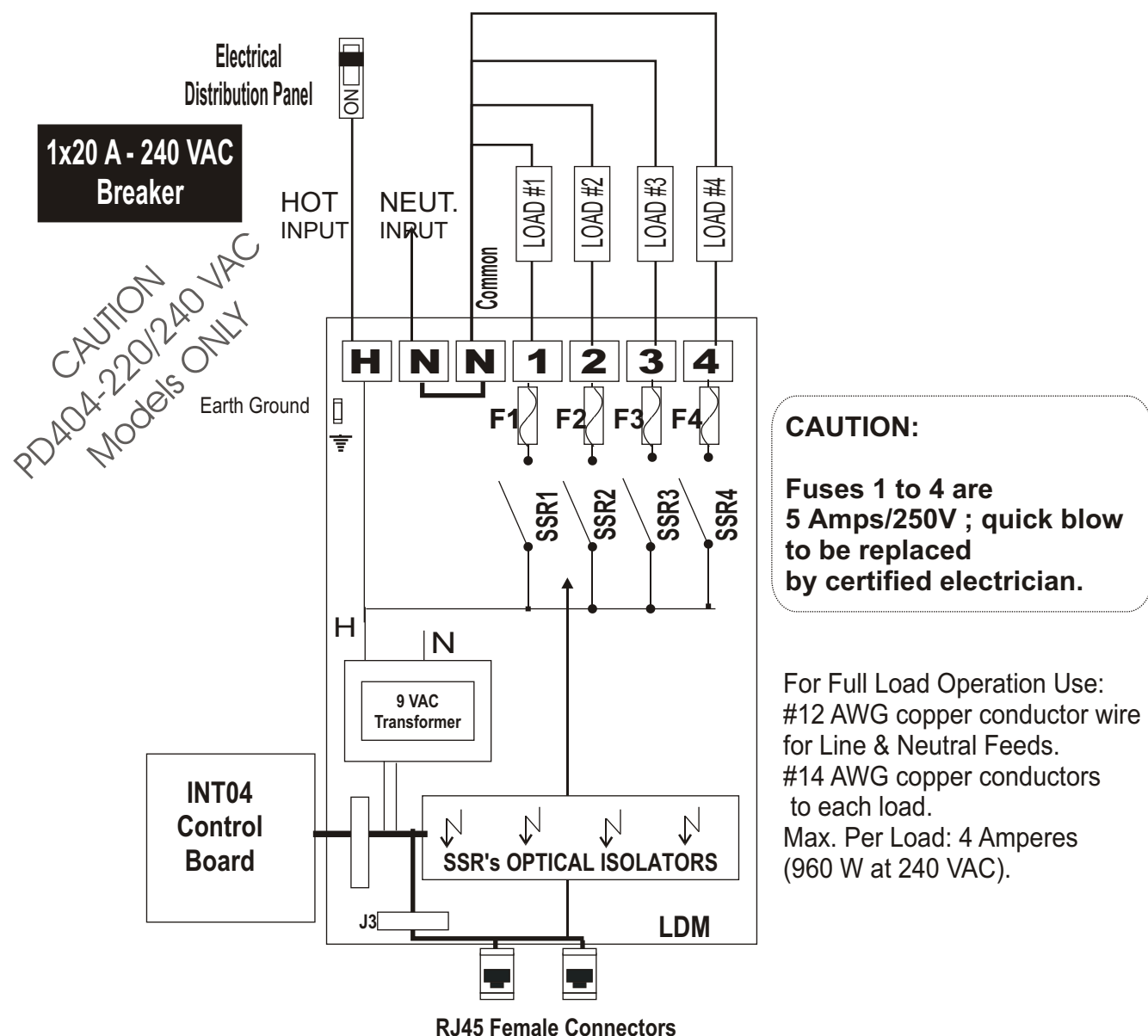
Figure 8 - PD404 Typical 220/240 VAC Wiring.
