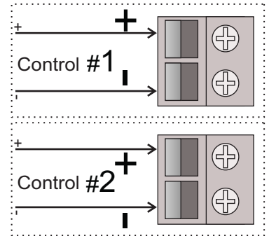
Figure 4 - PD216-AN10 Typical Control Wiring. Analog 0-10V Control inputs Compatible with sinking or sourcing standard 0-10V signals
