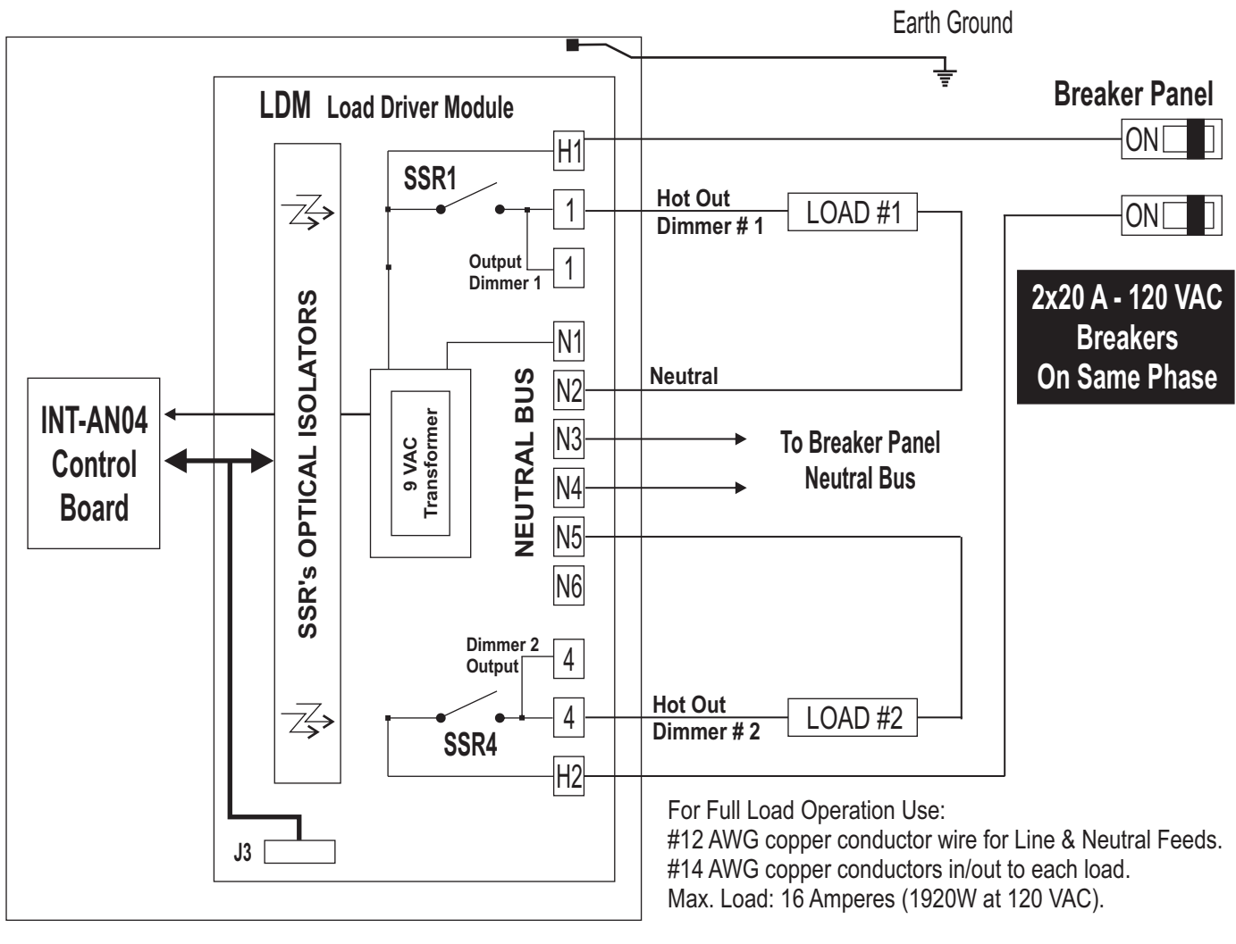
Figure 5 - PD216-AN10 Typical 120 VAC Wiring.
