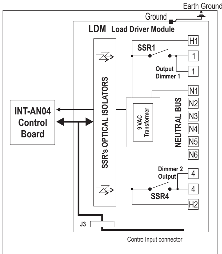
Figure 1 - PD216-AN10 LDM Detail
