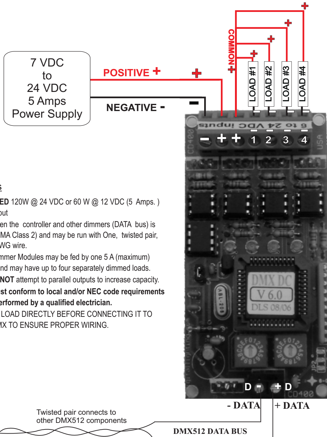
Figure 6 - CD400 GENERAL WIRING INSTRUCTIONS:
