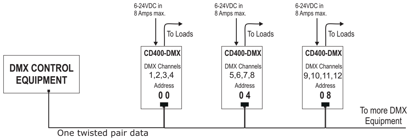
Figure 5 - Typical Installation
