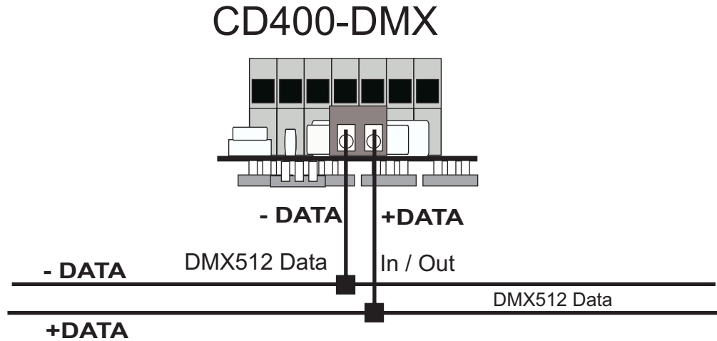
Figure 4 MD Dimmer Network Ports Connections.
